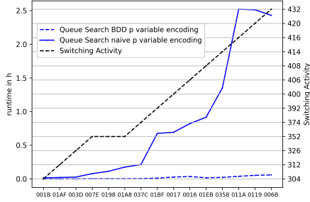
Figure 5: Runtime comparison of the p variable encoding strategy on Queue Search.
