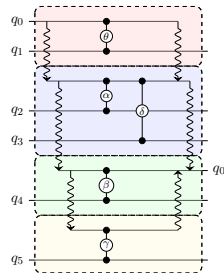
Distributed circuits
